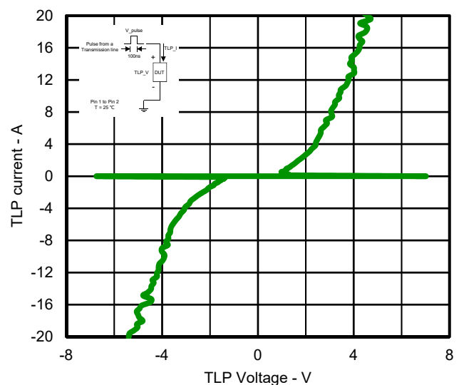
Fig.6 TLP Measurement
