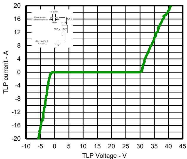
Fig.5 TLP Measurement
