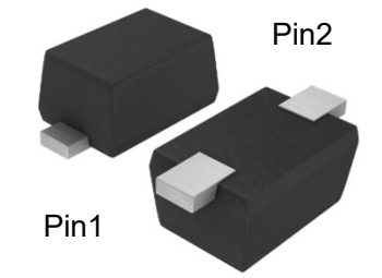
SOD-523
