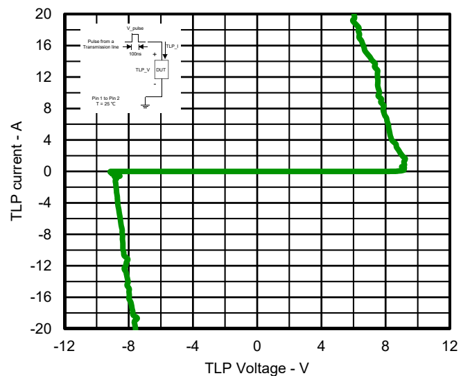
Fig.6 TLP Measurement
