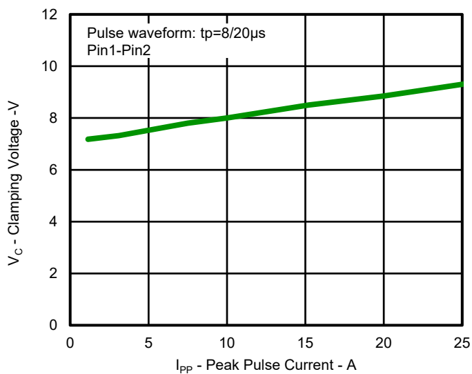
Fig.3 Clamping Voltage vs. Peak Pulse Current
