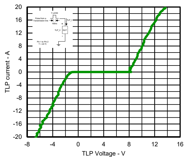
Fig.6 TLP Measurement
