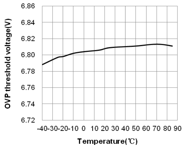
Figure 12. OVP threshold voltage vs. Temperature
