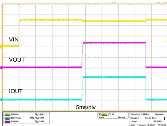
Figure 9. OCP Response at Start-up ( R_{load}=3\Omega , R_{lim}=5.6k\Omega )
