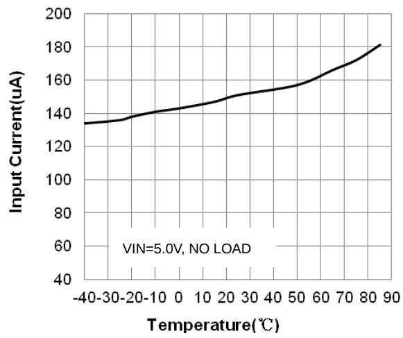
Figure 11. Input current vs. Temperature
