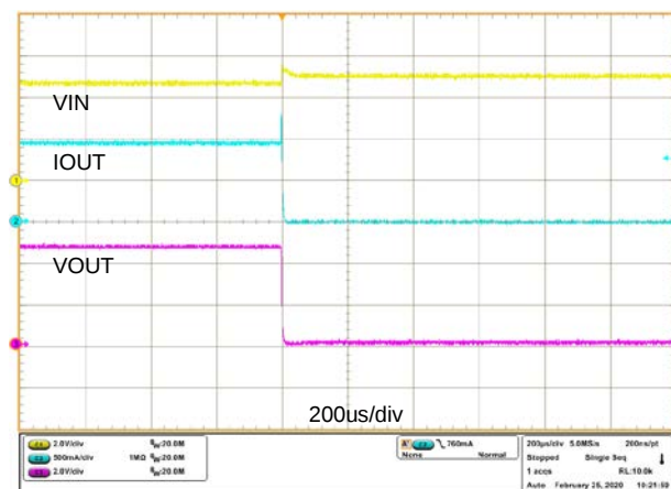
Figure 10. OCP Response after Start-up ( R_{load}=5\Omega to 3.5\Omega , R_{lim}=5.6k\Omega )
