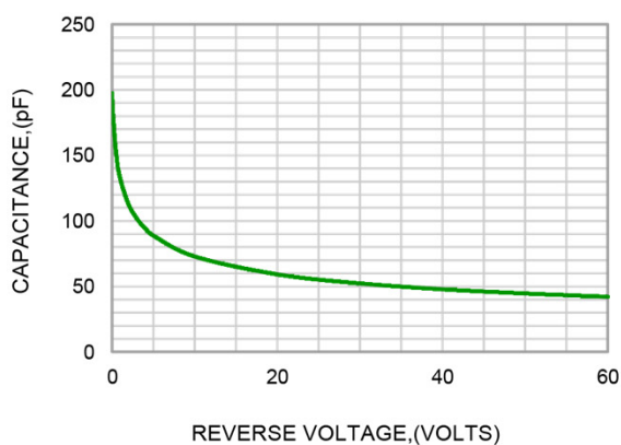
FIG.3-TYPICAL JUNCTION CAPACITANCE
