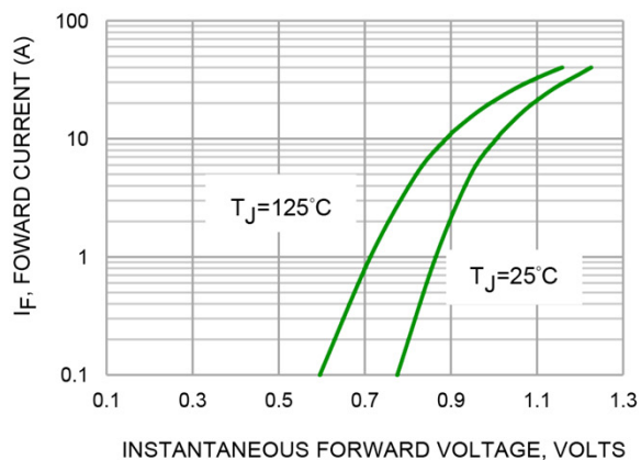
FIG.4-TYPICAL FORWARD CHARACTERISTICS
