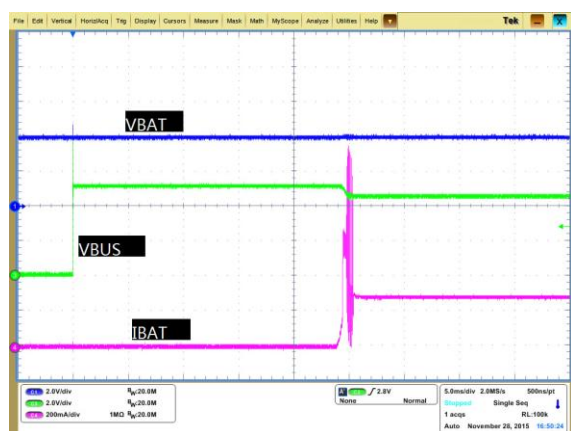
Figure 11. Auto-Charge Startup with 300mA Limited Charger/Adaptor, I_{INLIM}=500mA , V_{BAT}=3.9V
