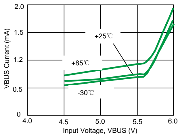
Figure 16. VBUS Current with Battery Open
