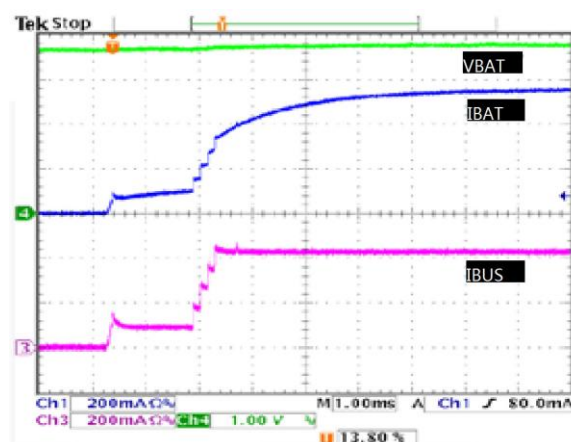
Figure 12. Charger Startup with HZ_MODE Bit Reset, I_{INLIM}=500mA , I_{OCHARGE}=956mA , O_{REG}=4.2V , V_{BAT}=3.6V
