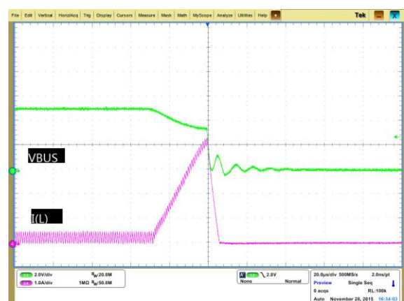
Figure 28. VBUS Fault Response, 3.6VBAT
