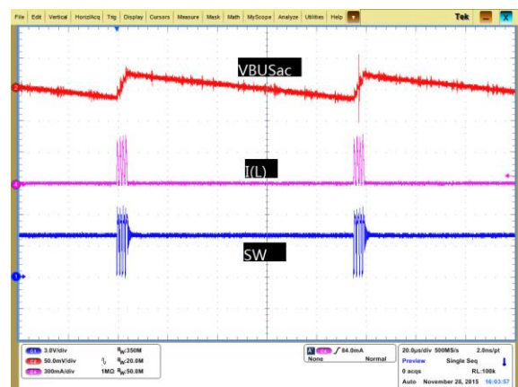
Figure 24. Boost PFM Waveform
