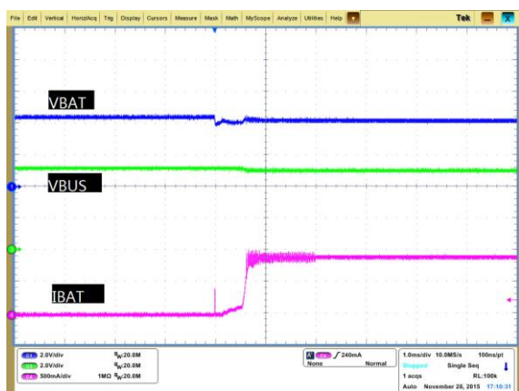
Figure 13. Battery Removal / Insertion during Charging, V_{BAT}=3.9V , I_{OCHARGE}=956mA , No I_{INLIM} , TE=0
