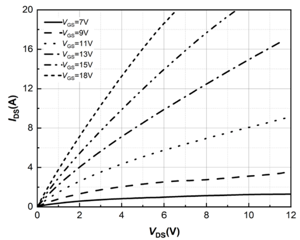
Figure 2 Output Characteristics
