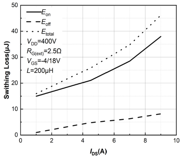
Figure 21. Clamped Inductive Switching Energy vs. Drain Current
