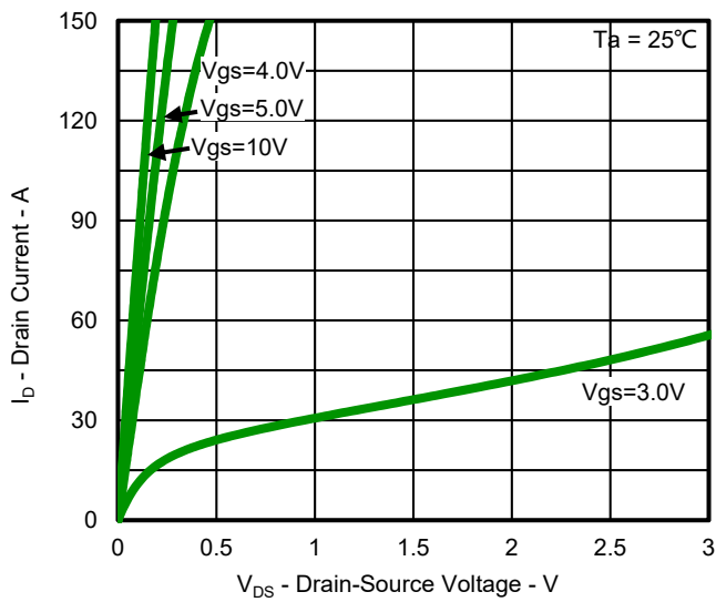
Fig.1 Output Characteristics
