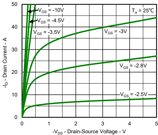
Fig.1 Output Characteristics
