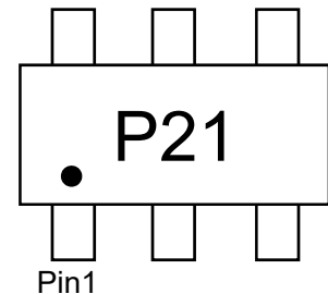
Marking (Top View)
