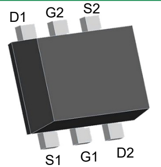
SOT-563 (Top View)
