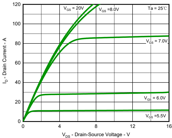
Fig.1 Output Characteristics
