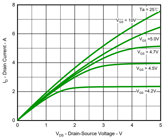
Fig.1 Output Characteristics
