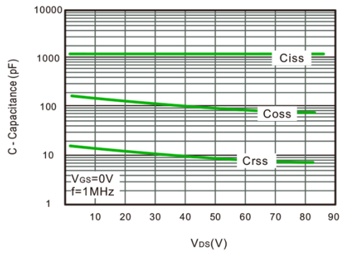
Fig.9 Capacitance Characteristics
