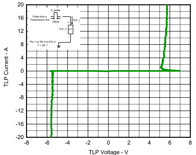
Fig 6. TLP Measurement
