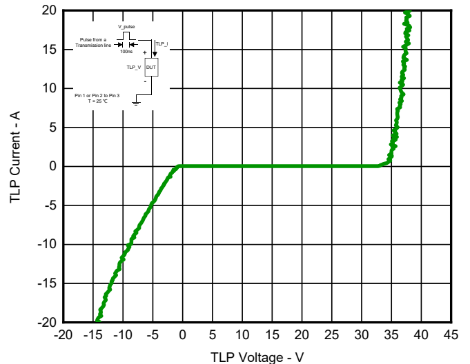
Fig 6. TLP Measurement
