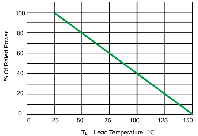
Fig 2.Power Derating Curve
