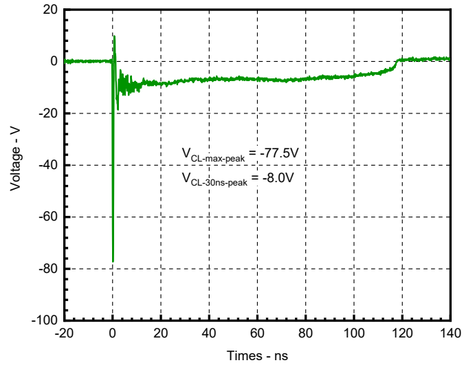
Fig 8. Clamping Voltage at IEC61000-4-2 -8kV Pulse Waveform
