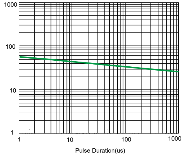
Fig 6. Non-Repetitive Peak Pulse Power vs. Pulse time
