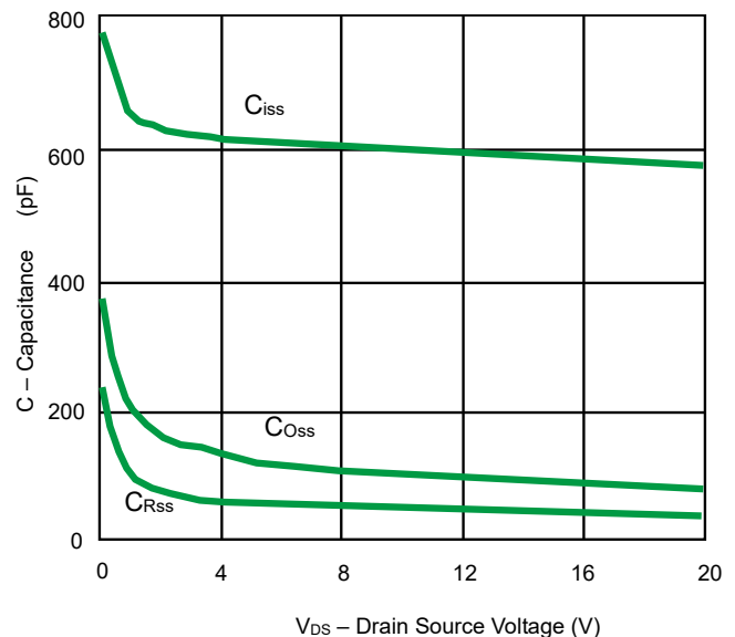
Fig 4. Capacitance
