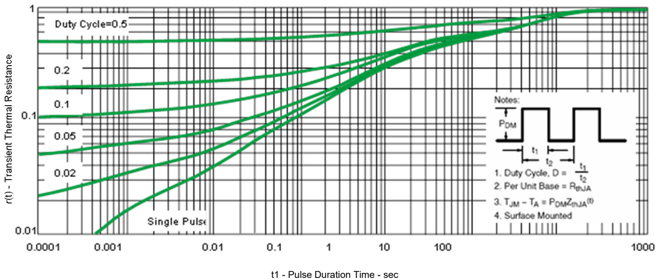
Fig.10 Transient Thermal Resistance
