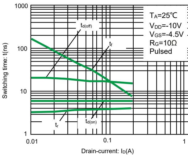
Fig 11. Switching characteristics
