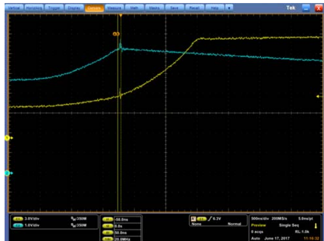
Figure 5. OVP response
