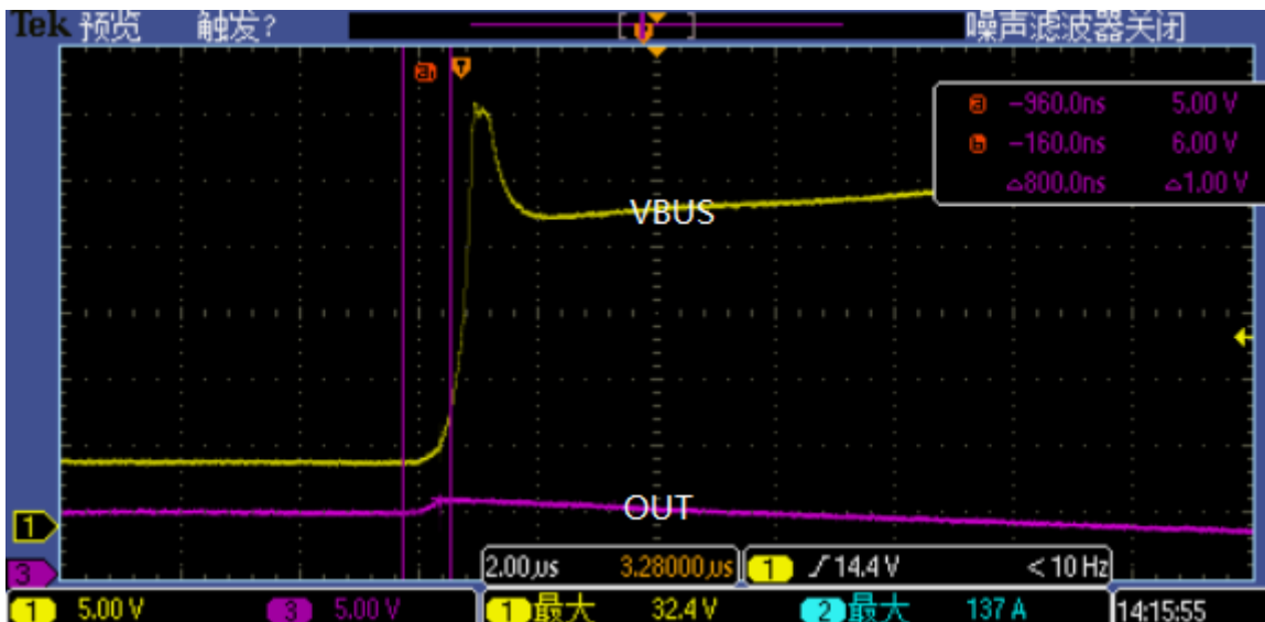
Figure 8. 8-20 Surge test (Base on Schematic, Figure7)
