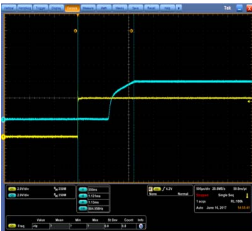
Figure 4. Start-up waveform
