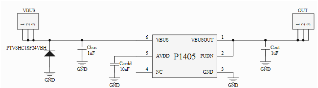
Figure 7. OVP test schematic
