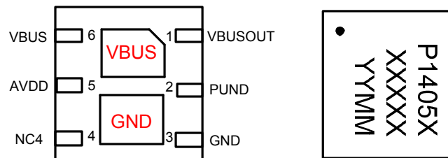
Figure 2. Pin order (Bottom view) and Marking (Top view)
